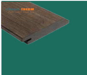
S0 QH-1 Charcoal, Unfinished Shiplap Cladding T18 * W75 * L1850/2000/2440 mm T18 * W137 * L1850/2000/2440 mm
