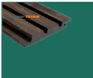
S0 QH-3 Charcoal, Unfinished Triple Rhombus Cladding T20 * W137 * L1850/2000/2440 mm
